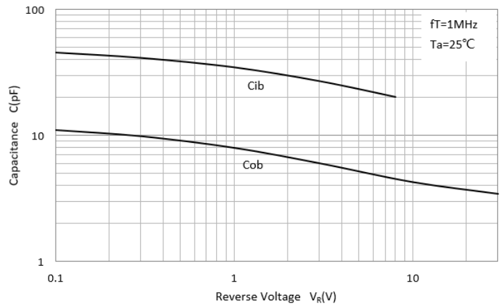
Cob/Cib-VCE/VEB
