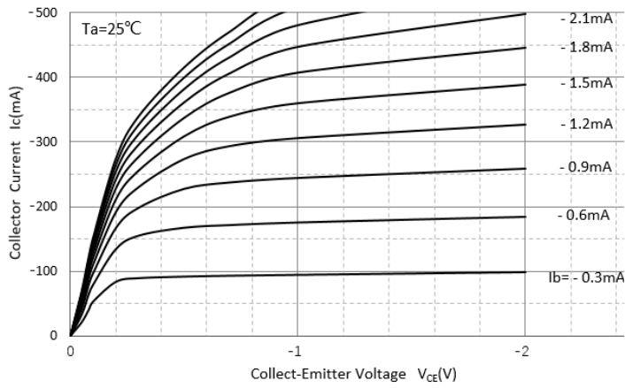
Static Characteristic
