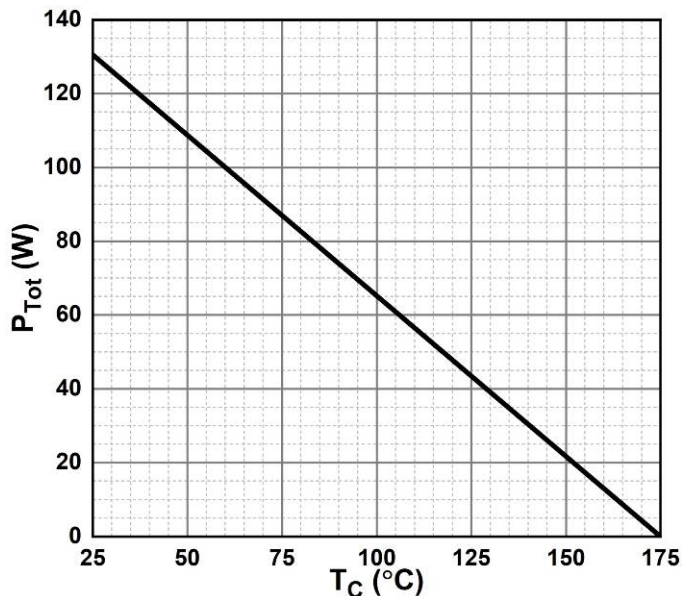
Figure 6. Power Derating
