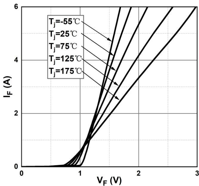
Figure 1. Forward Characteristics
