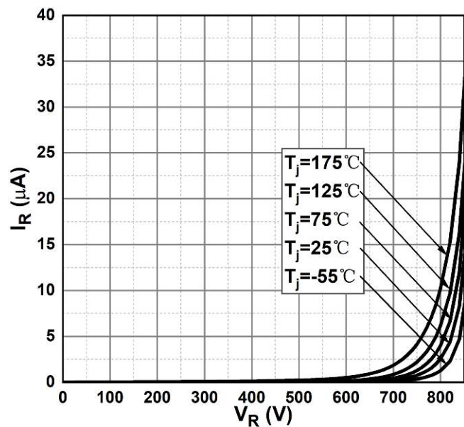
Figure 2. Reverse Characteristics
